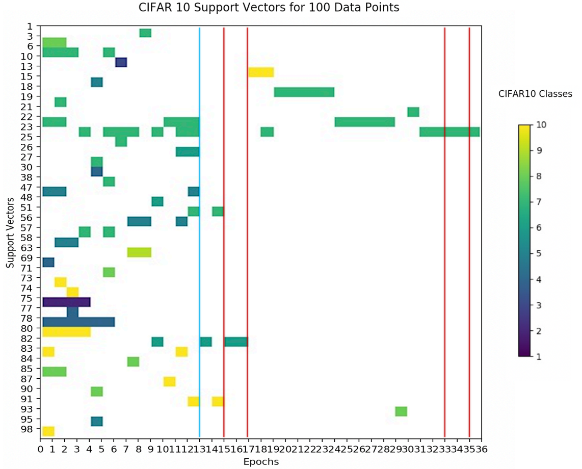
Figure 10: Datapoints closest to the margin solution (support vectors). A 5-layer convolutional neural network was trained on 100 data points from the CIFAR10 dataset as in Figure 9, the blue line represents data convergence (100 % accuracy training). Support vectors were obtained by taking the smallest of the distances between the class output and the second highest class output for each datapoint, \text{argmin}(f_{y_i} - \max_{j \neq i} f_{y_j}) . After convergence, perturbations to the network were performed with respect to the gradient of each individual weight, 0.5 \|\Delta_w L\| . The network converges to either one support vector or a set of support vectors when trained on more datapoints. Depending on the perturbation, the network converges to a different set of support vectors or comes back to the same one.
