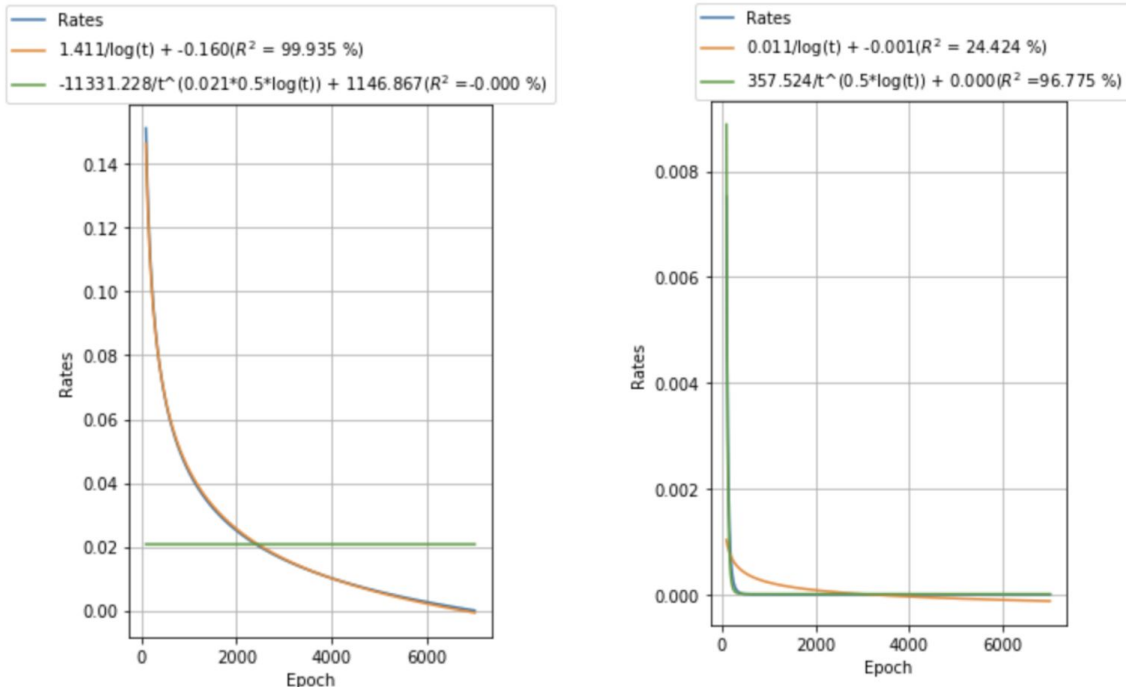
Figure 4: Rates of convergence of v(t) for a linear network trained on 1 training example on the IRIS dataset. Left: Standard gradient descent converges in direction at the rate \mathcal{O}(\frac{1}{\log t}) . Right: Weight Normalization changes the convergence rate to that of \mathcal{O}(t^{-1/2} \log t) . We obtain more complex behavior in the presence of multiple support vectors with different margins.
