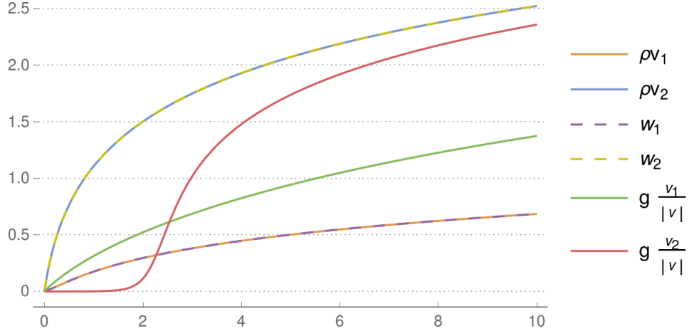
Figure 2: Example comparison of dynamics \dot{W}_k = -\frac{\partial L}{\partial W_k} (dashed lines) and their equivalence to the reparametrization of the unconstrained dynamics (orange and blue) as a function of time. Standard weight normalization leads to different trajectories of gradient descent (in green and red). The example is that of a linear network with only two parameters and two training examples, using an exponential loss.
