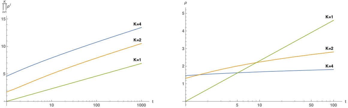
Figure 3: The left graph shows how the product of weights \prod_{i=1}^K scales as the number of layers grows when running gradient descent with an exponential loss. In the 1-layer case we have \rho = \rho \sim \log t , whereas for deeper networks the product of norms grows faster than logarithmically. As we increase the number of layers, the individual weights at each layer diverge slower than in the 1-layer case, as seen on the right graph.
