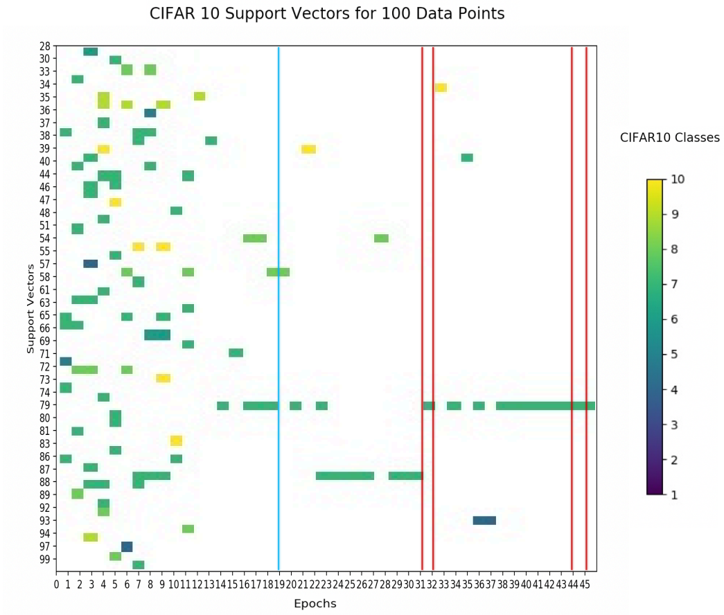
Figure 11: Same experiment as Figure 10 with different perturbation size 0.9 \|\Delta_w L\| .
